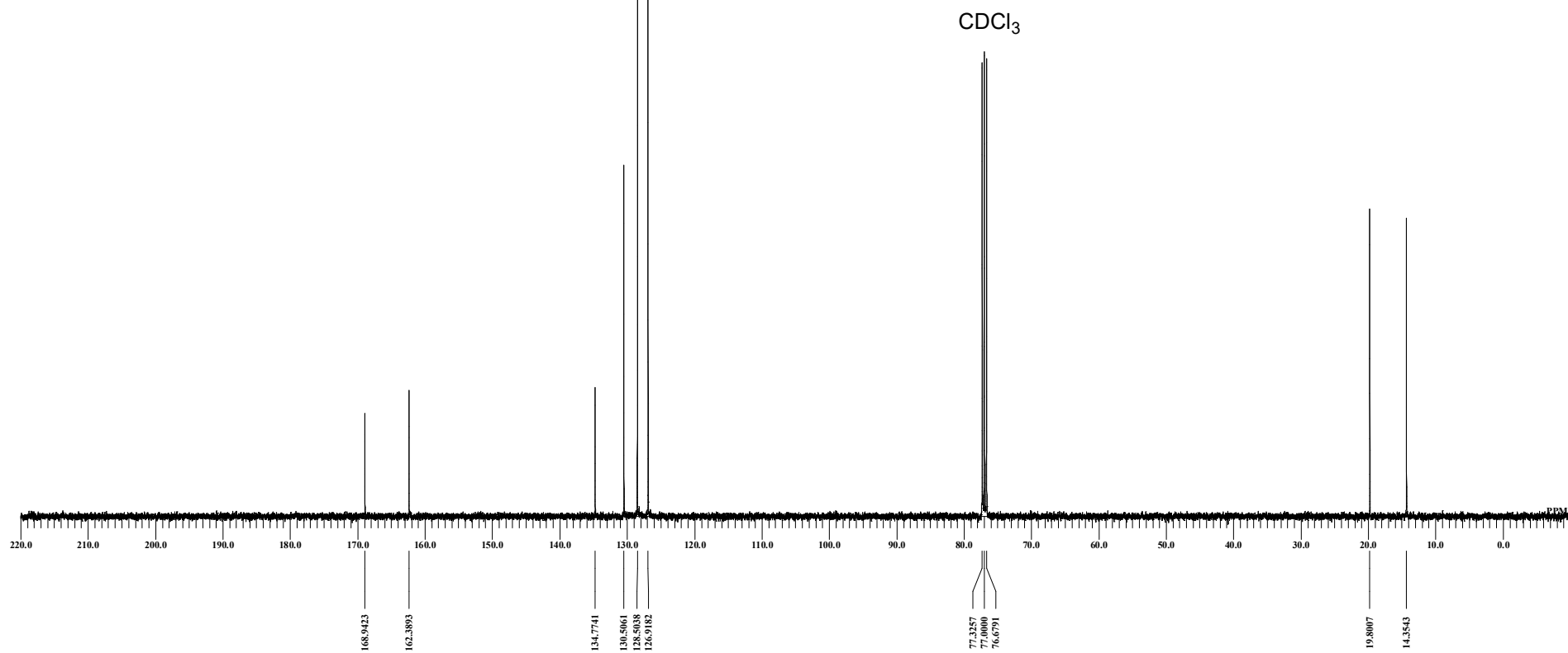
Acetophenone O -acetyl oxime ( 3 ) ^{13}\text{C} NMR (100 MHz, \text{CDCl}_3 )
